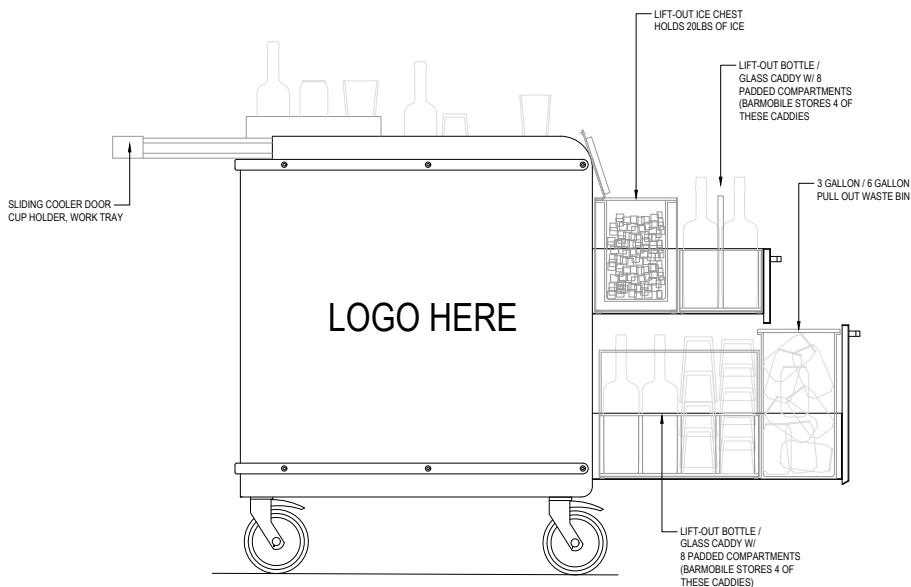
SIDE VIEW DRAWERS OPEN COOLER OPEN
