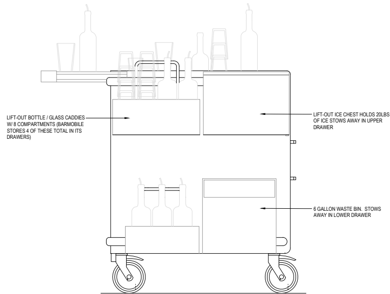
REAR VIEW
